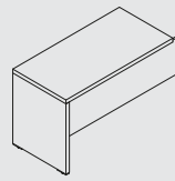
MIT12 1200 | 600 | 740 47 1/4" | 23 5/8" | 29 1/8"
