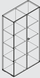
MIT15 916 | 418 | 1661 36 1/8" | 16 1/2" | 65 3/8"
