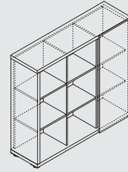
MIT7 1400 | 422 | 1280 55 1/8" | 16 5/8" | 50 3/8"
